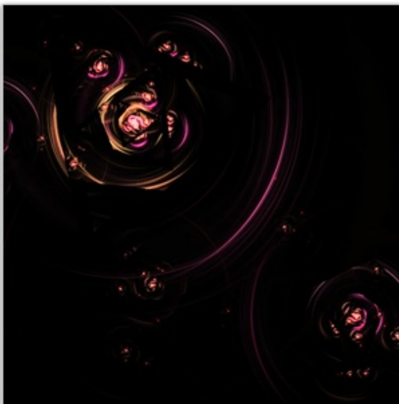
Triangular Trap in Subspace
