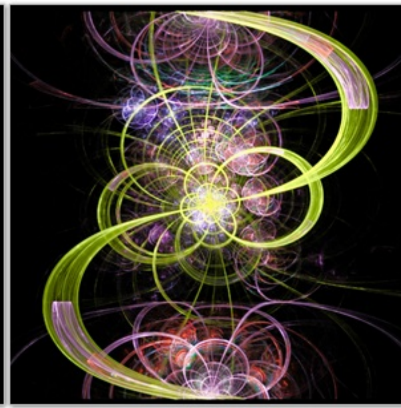
Encryption
